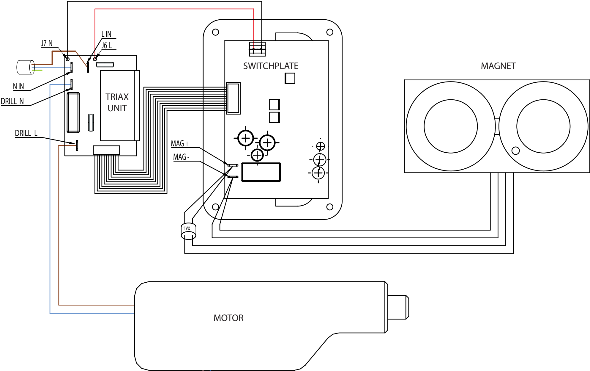
Magtron MB30 Electronic Switchplate (MM2) Wiring Diagram - Dual Voltage
